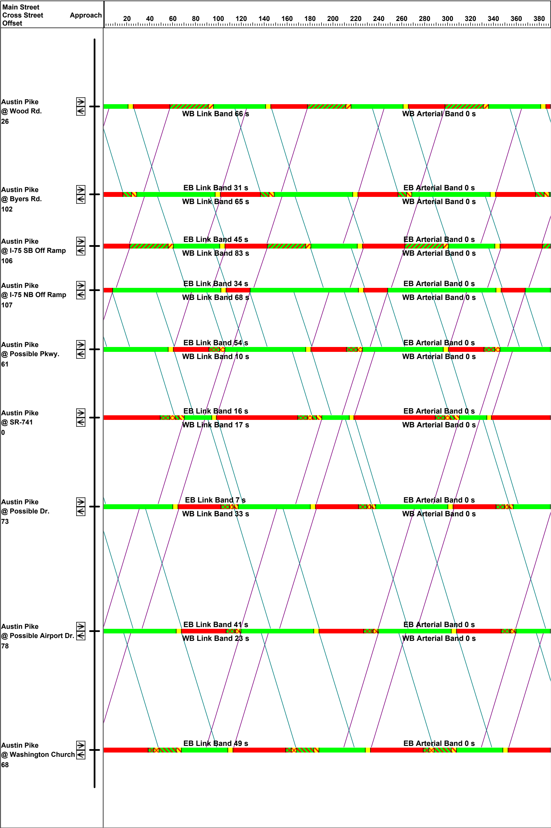
Figure 4B - Analysis Of Possible Signals With TSM And An Interchange PM - Worse Case
