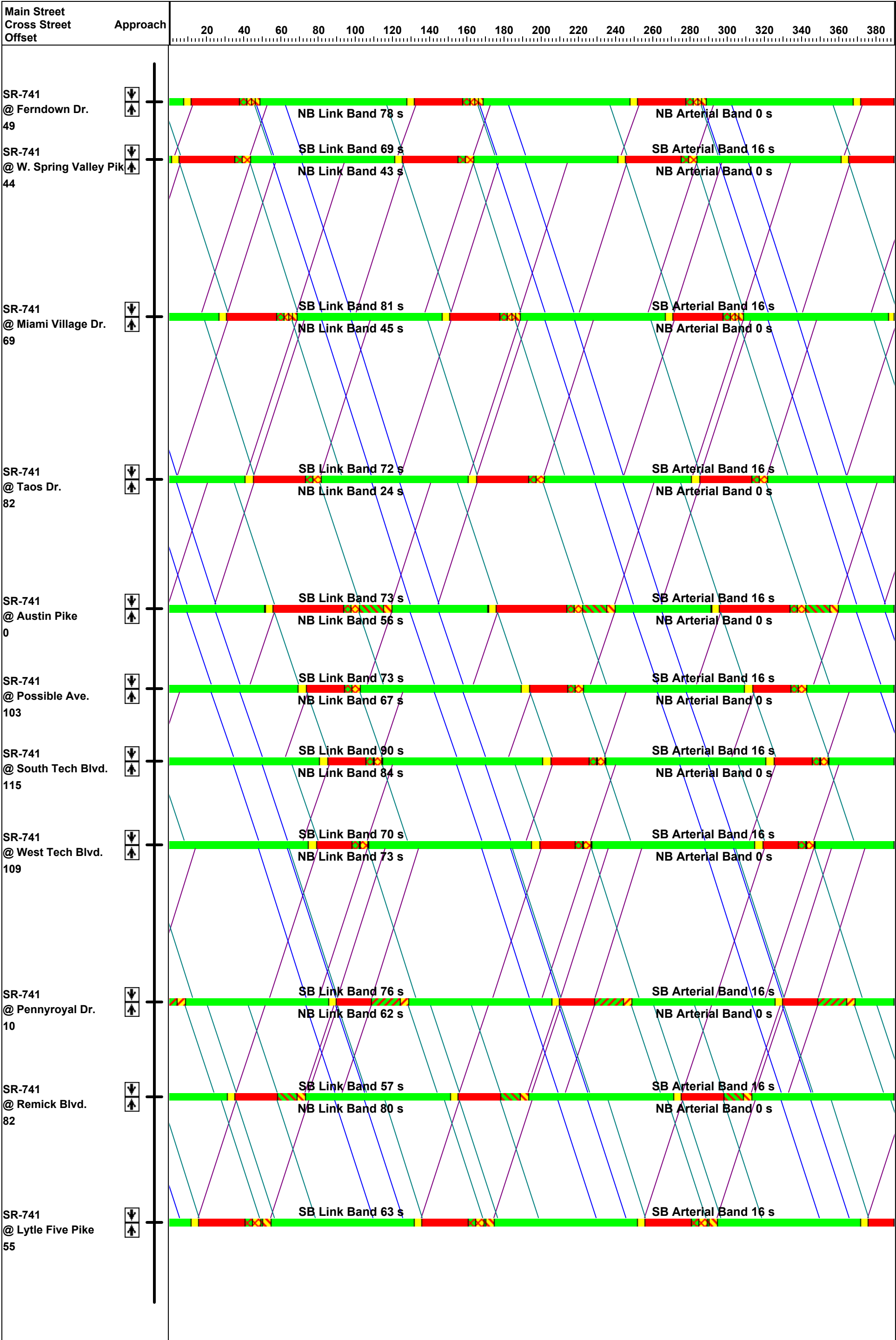
Figure 3A - Analysis Of Possible Signals With TSM No Interchange PM - Worse Case
