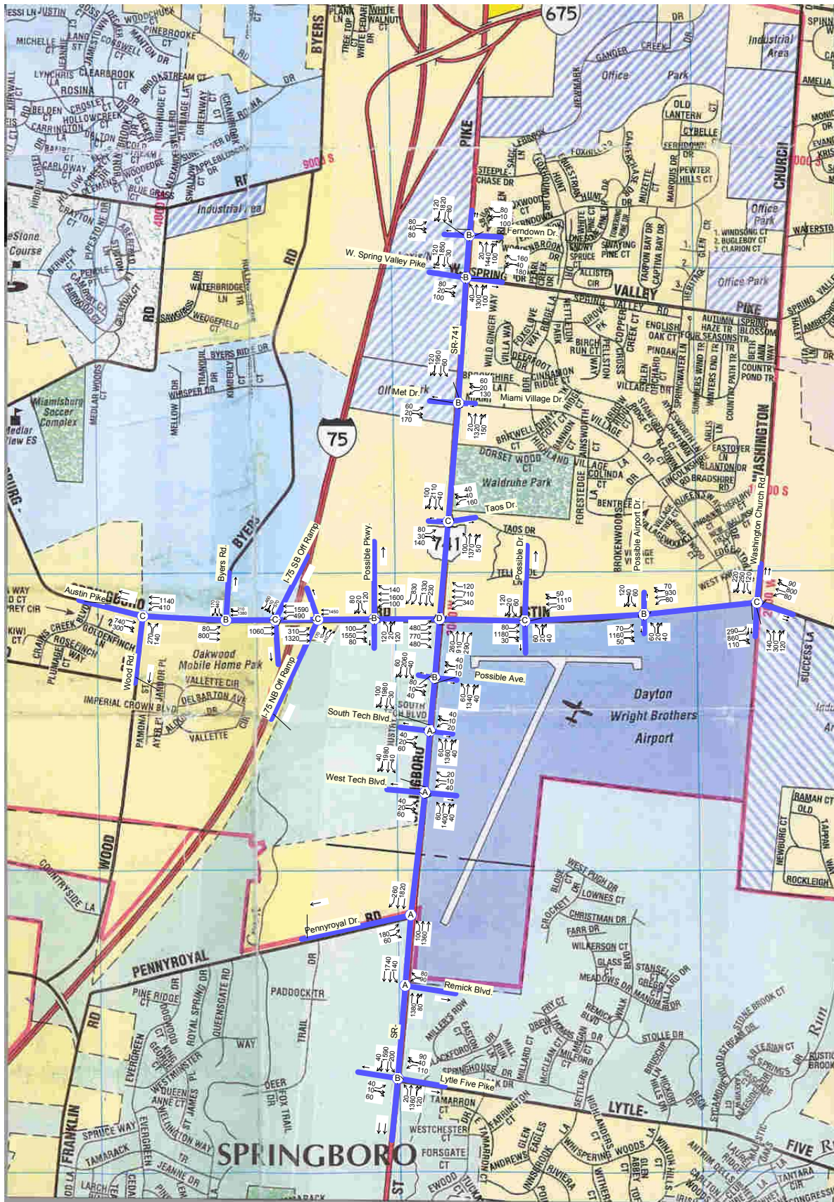
Figure 4 - Analysis Of Possible Signals With TSM And An Interchange PM - Worse Case
