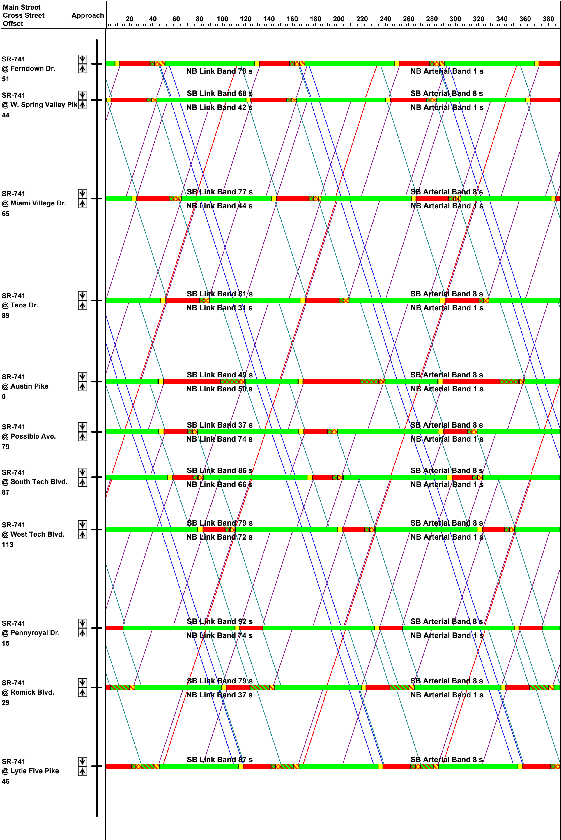
Figure 4A - Analysis Of Possible Signals With TSM And An Interchange PM - Worse Case
