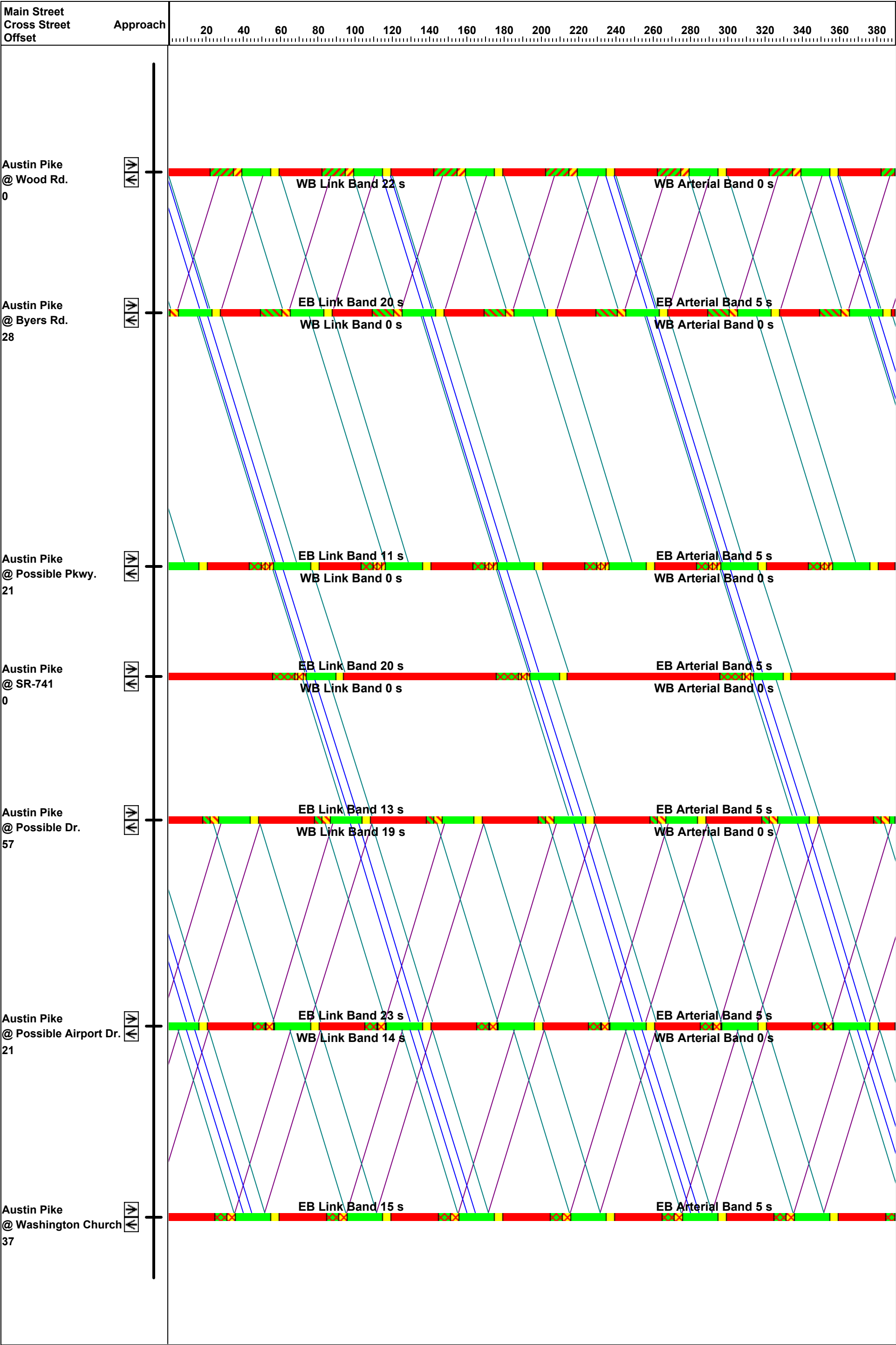
Figure 3B - Analysis Of Possible Signals With TSM No Interchange PM - Worse Case
