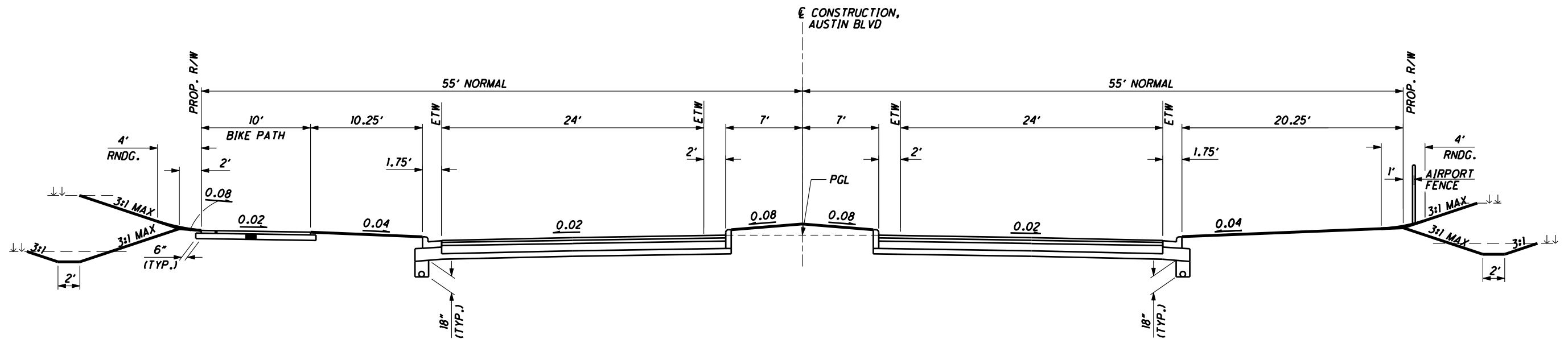
NORMAL SECTION - AUSTIN BLVD
